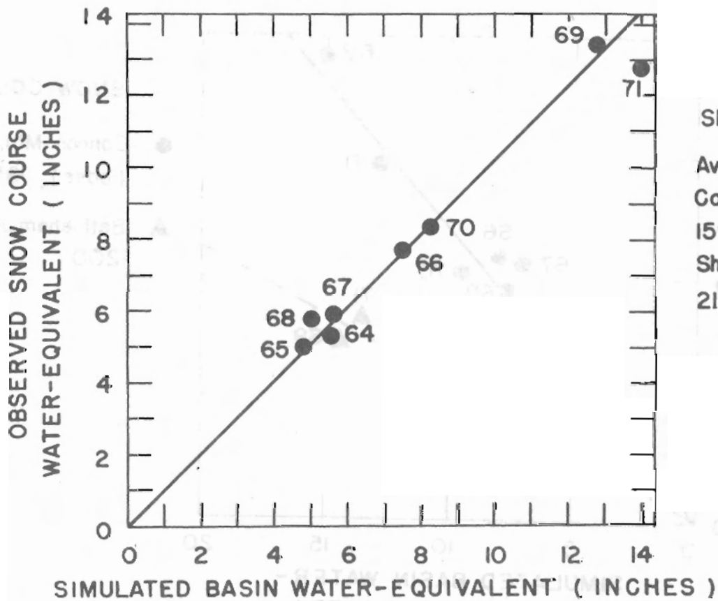
Figure II - Spring runoff (March-May) and water-equivalent comparisons, White River
