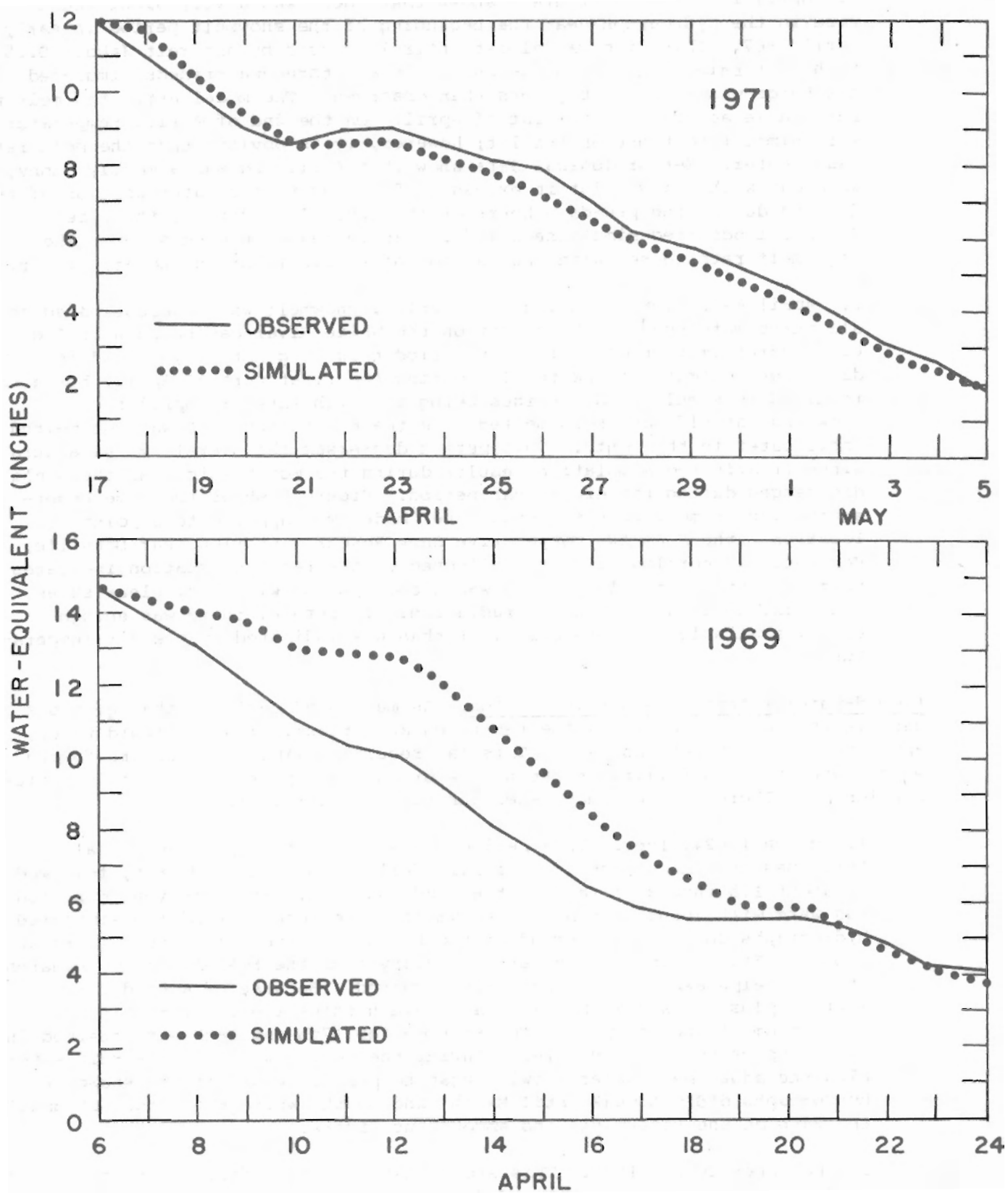
Figure 9 - Simulation of snow pillow data-NOAA-ARS Cooperative Snow Research Station, Danville, Vt.
