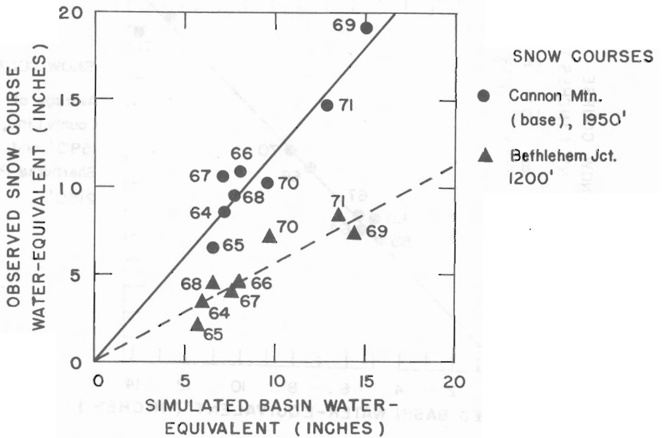
Figure 10 - Spring runoff ( March-May ) and water-equivalent comparisons, Ammonoosuc River
