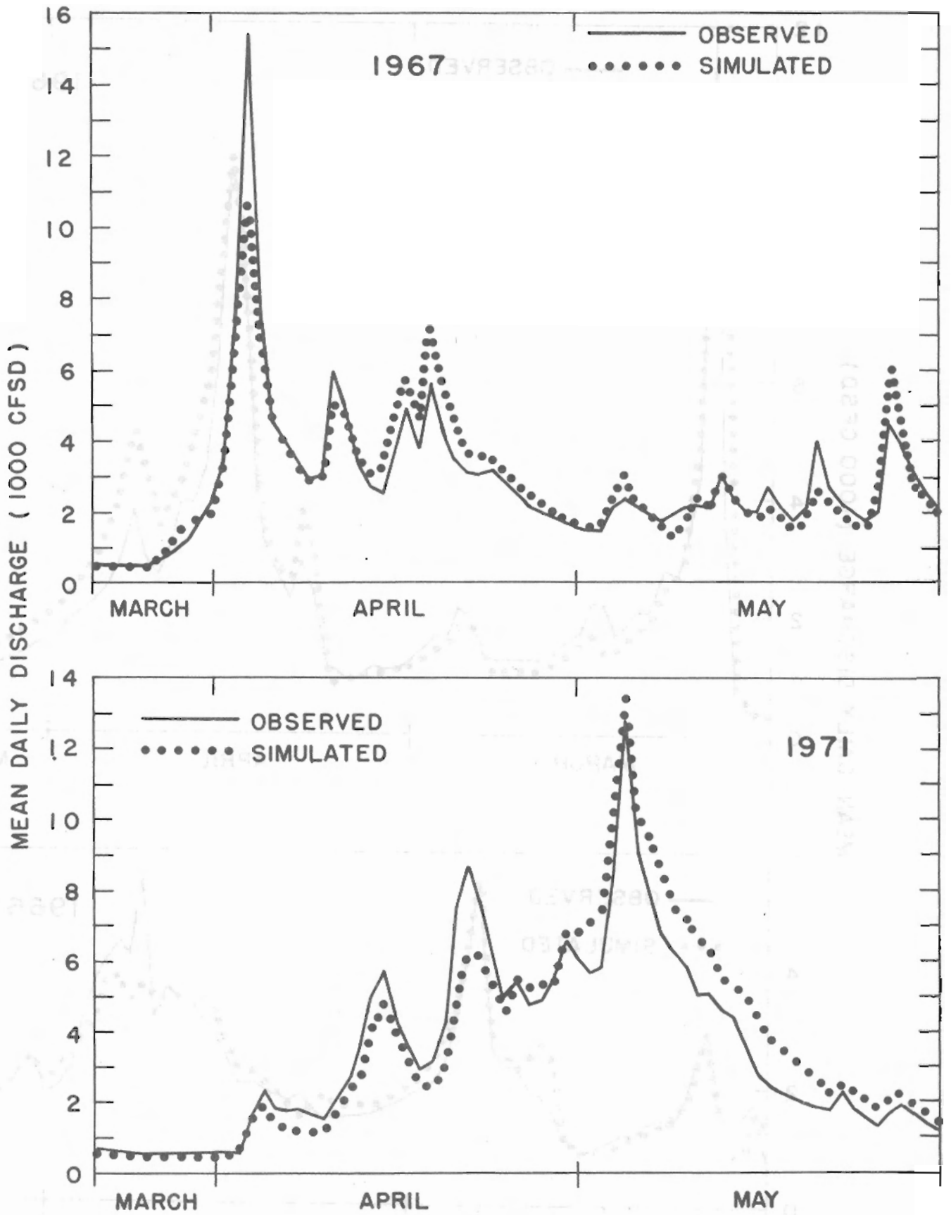
Figure 5 - White River hydrographs
