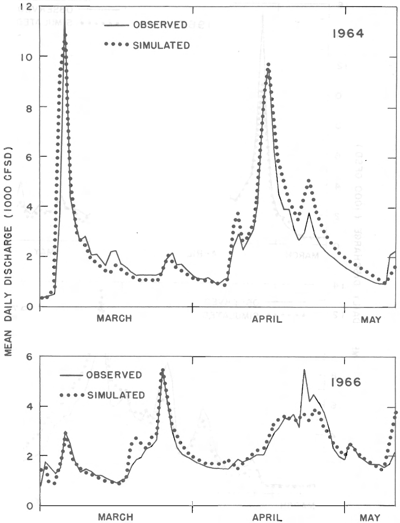
Figure 4 - White River hydrographs.
