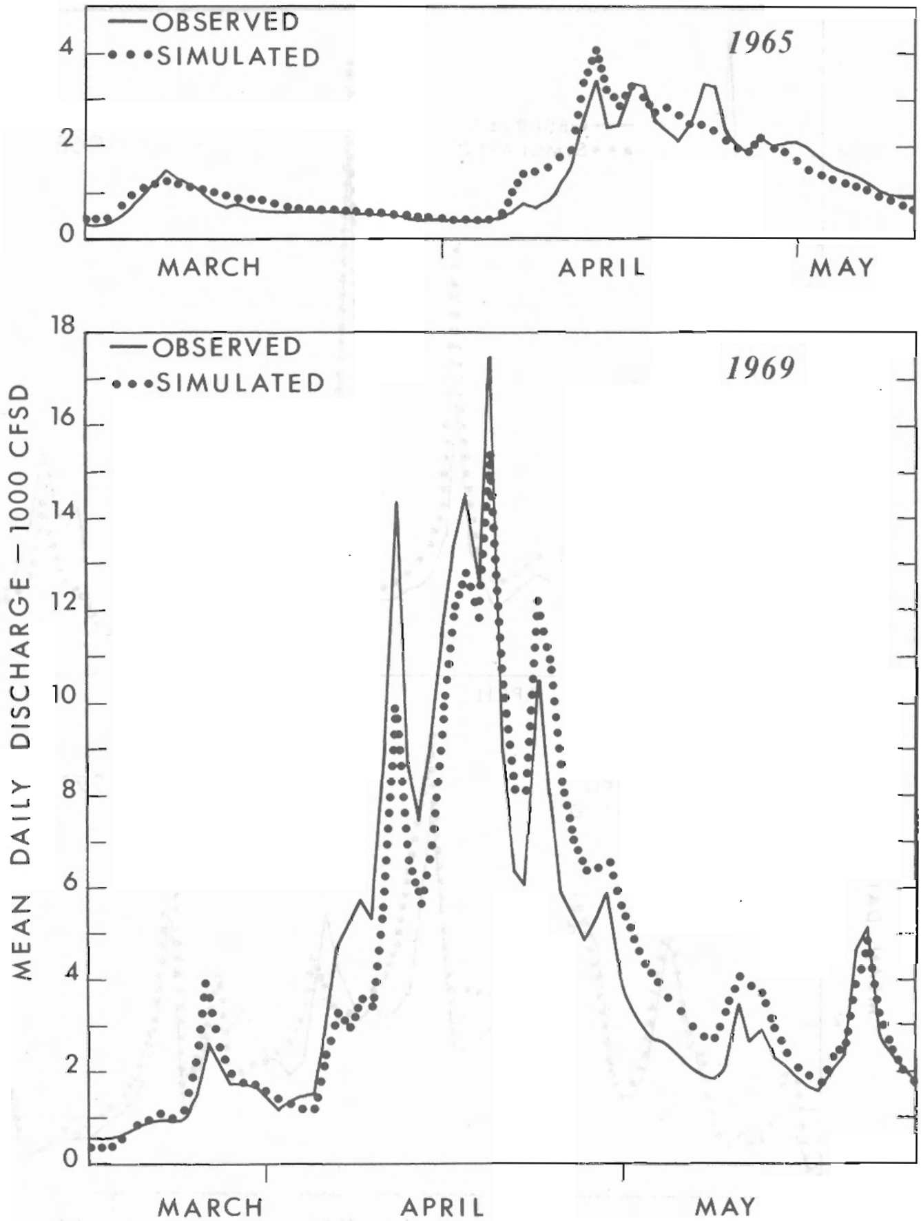
FIGURE 6 -- WHITE RIVER HYDROGRAPHS.
