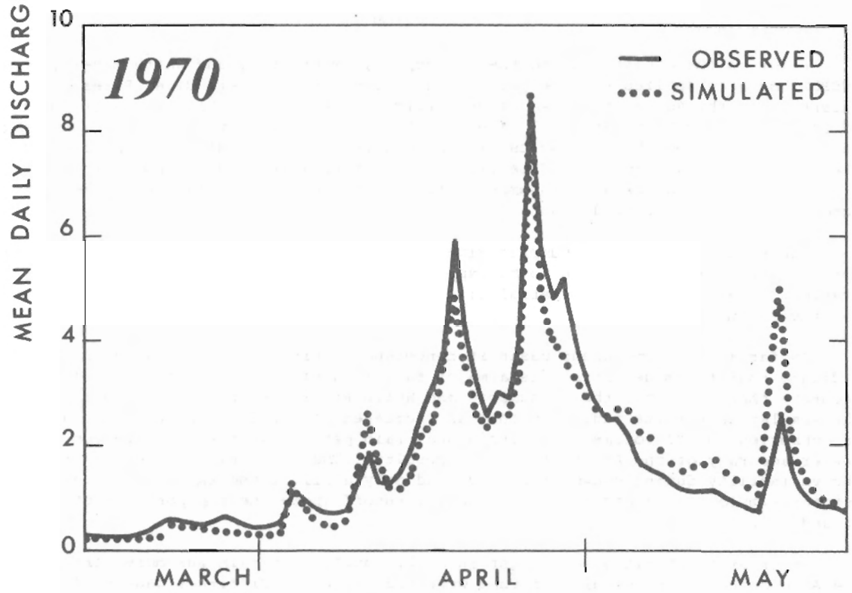
FIGURE 3 — PASSUMPSIC RIVER HYDROGRAPHS
