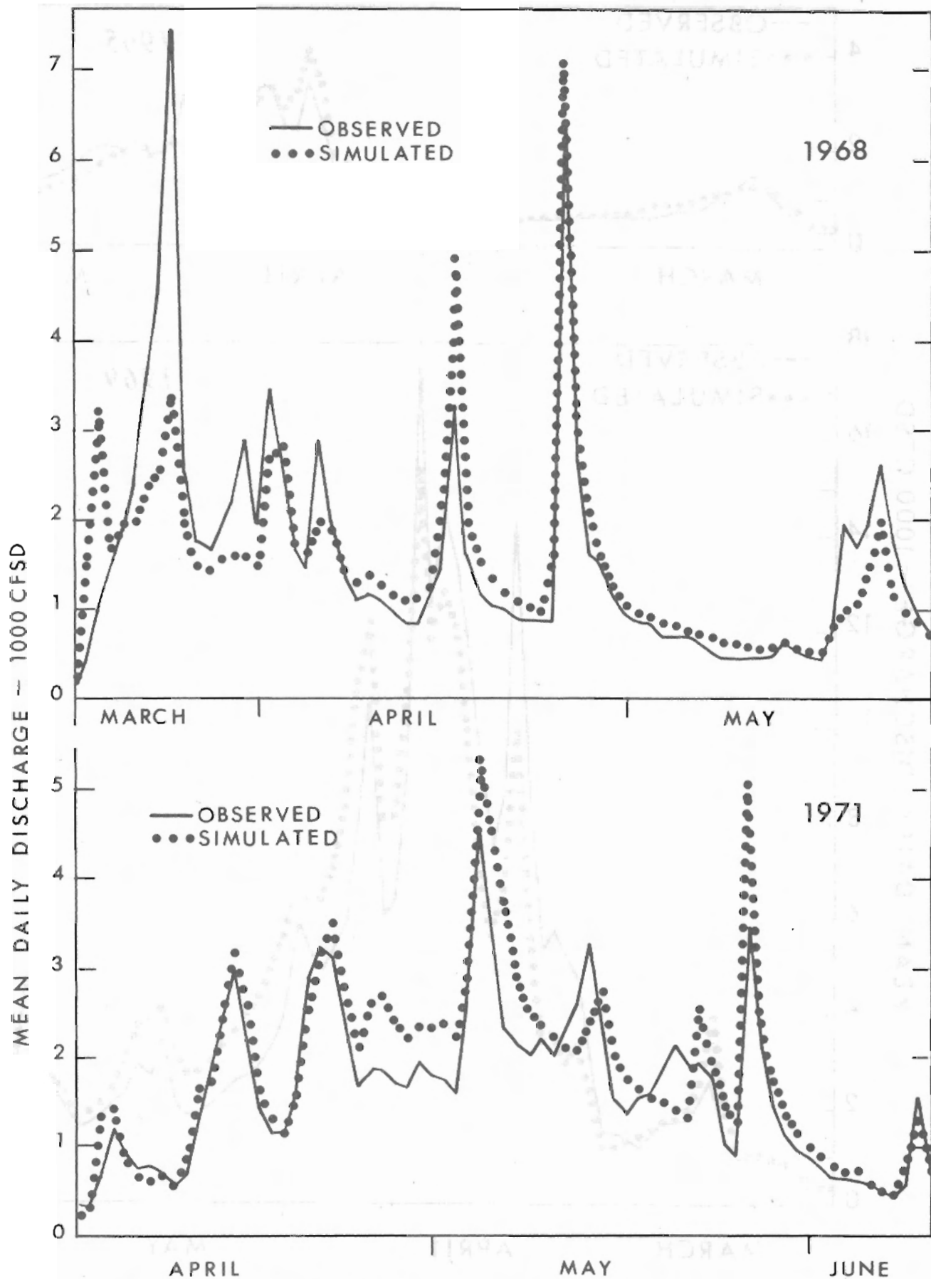
FIGURE 7 - AMMONOOSUC RIVER HYDROGRAPHS.
