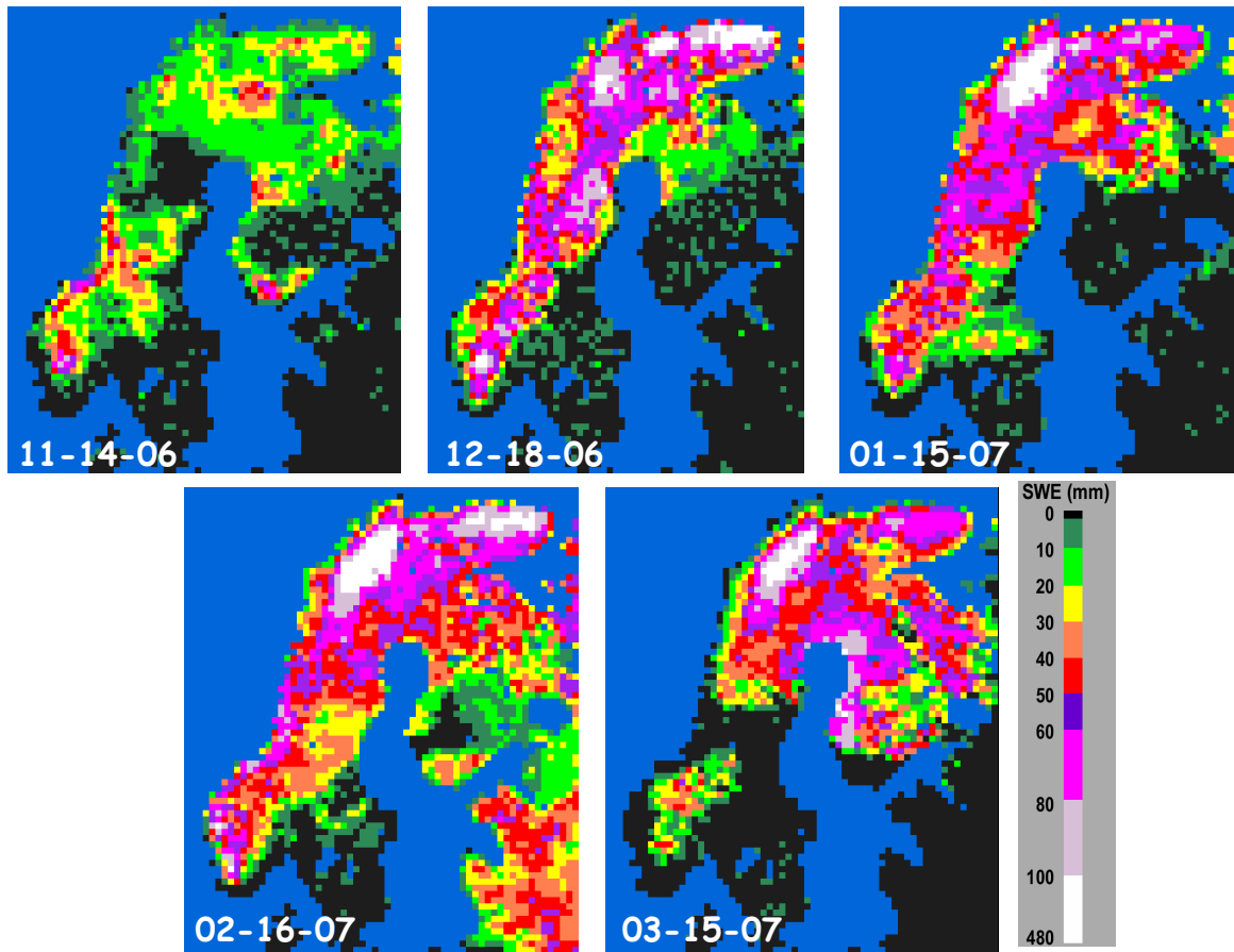
Figure 4a. AMSR-E SWE maps for all of Scandinavia for the snow course comparison dates in November 2006 through March 2007.
