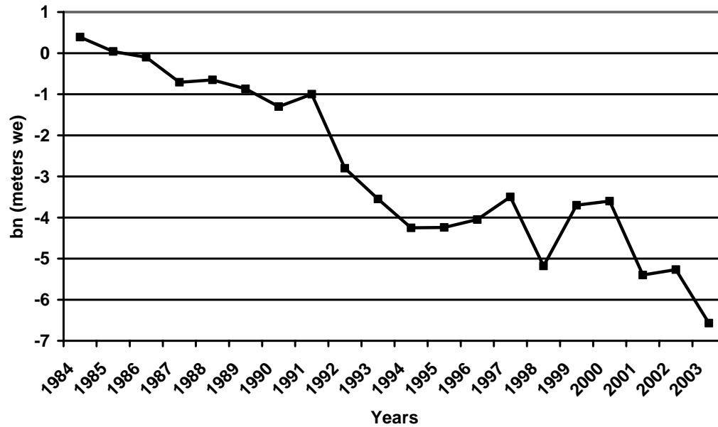
Figure 7. Cumulative annual balance on eight North Cascade glaciers observed by the NCGCP (Pelto, 1996; Pelto and Riedel, 2001).
