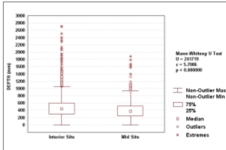
Figure 5. Snow depth at the Interior and Mid Site.
