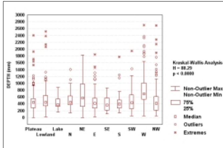
Figure 6. Snow depth by terrain class, Interior Site.
