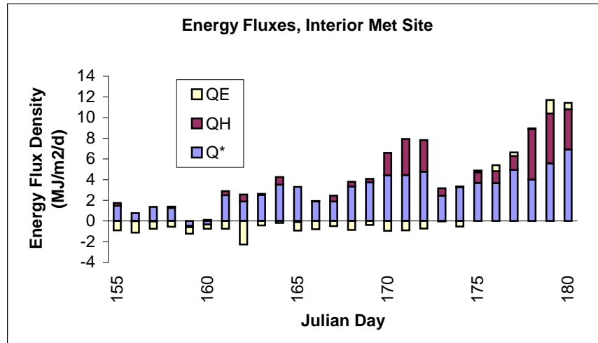
Figure 7. Energy fluxes at the Interior Site meteorological station, Julian Day 155 to 180 (June 3 to June 28).
