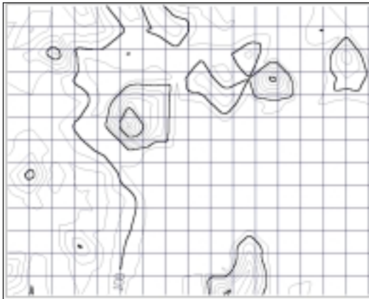
Figure 8. Predicted SWE values (60-190mm), Julian Day 168. Contour interval = 10 mm.
