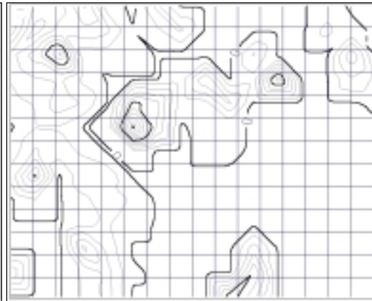
Figure 9. Predicted SWE values (0-100mm), Julian Day 173. Contour interval = 10 mm.
