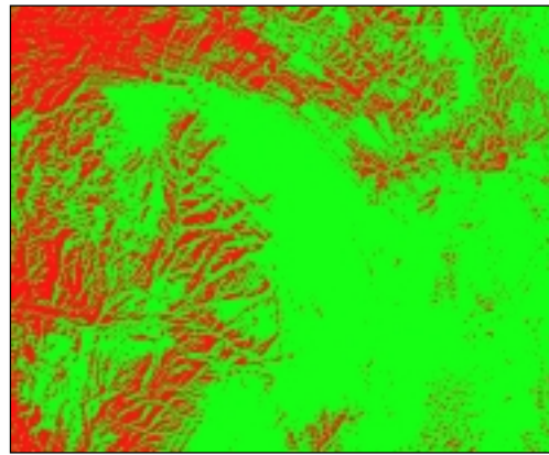
Figure 11. Classified Landsat-7 pan scene, Julian Day 173, Interior Site. Lighter tone is snow cover, darker tone snow free.
