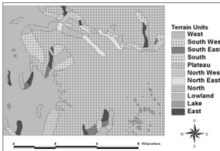
Figure 3: Revised landscape classification map.
