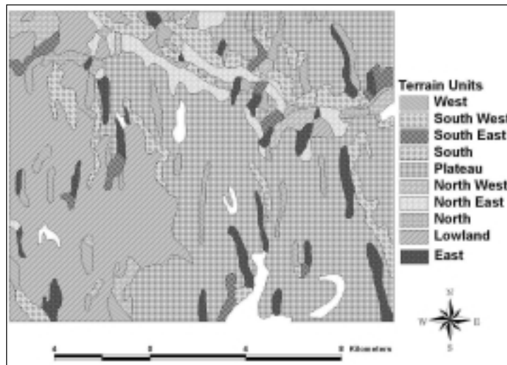
Figure 2. DEM-derived landscape classification map.
