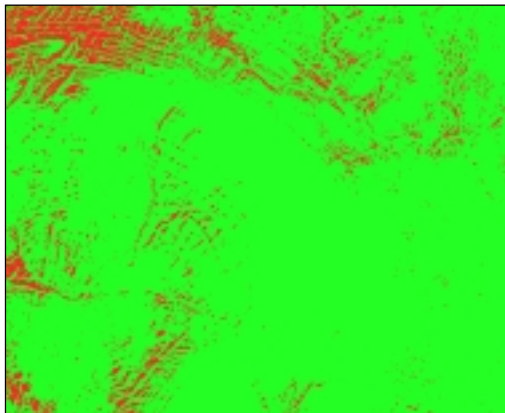
Figure 10. Classified Landsat-7 pan scene, Julian Day 168, Interior Site. Lighter tone is snow cover, darker tone snow free.
